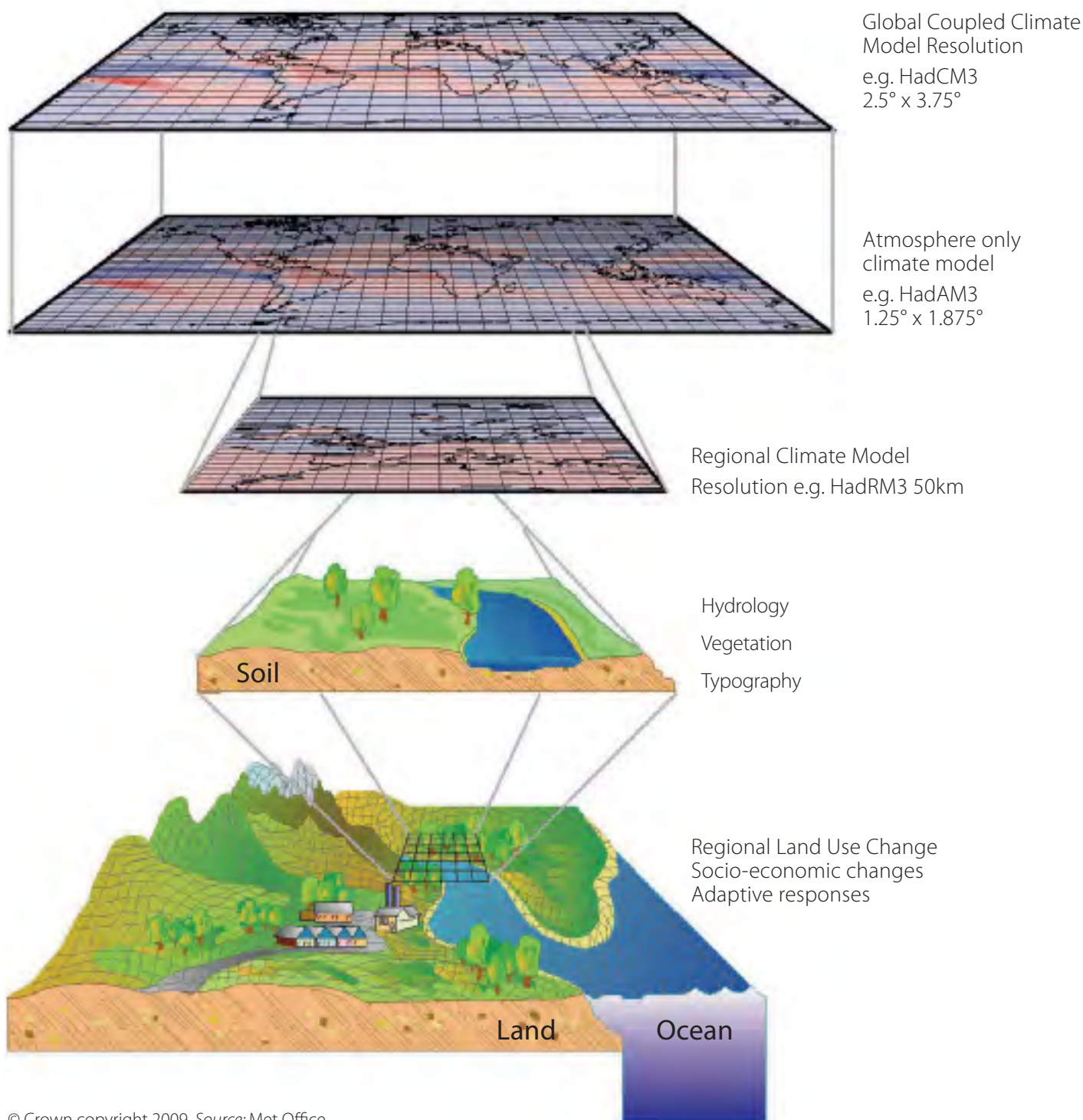
Figure 7: Dynamic downscaling
