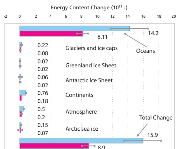
Figure 2 The change in energy content in different components of the Earth System for two periods: 1961-2003 (blue bars) and 1993-2003 (pink bars) 2 (figure 5.4).
