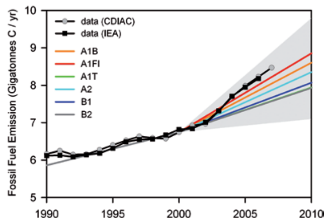
Observed global fossil-fuel and industrial CO 2 emissions 18 , compared with averages of 6 scenario groups from the IPCC Special Report on Emissions Scenarios (coloured lines) and range covered by all individual scenarios (grey shading). Emission data are from two sources: The Carbon Dioxide Information and Analysis Center (CDIAC) and the International Energy Agency (IEA). Figure updated using the latest available data ( www.globalcarbonproject.org ) since the original publication of this report.
